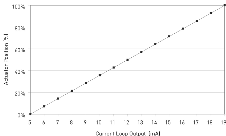
Figure 4.4: Position Control
