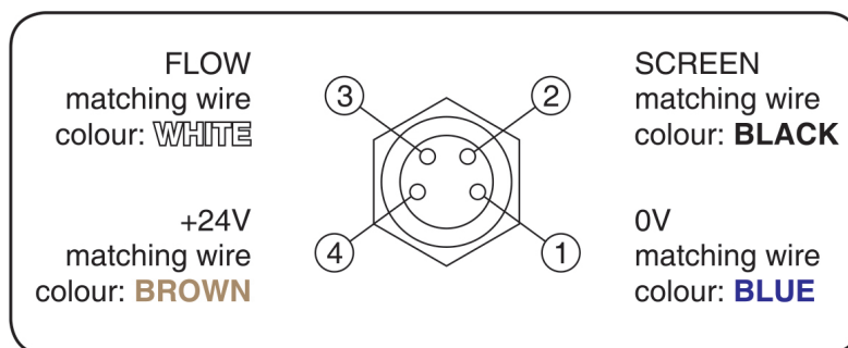
Figure 3.9: Auxiliary input on M8 male connector (PORT-2)
