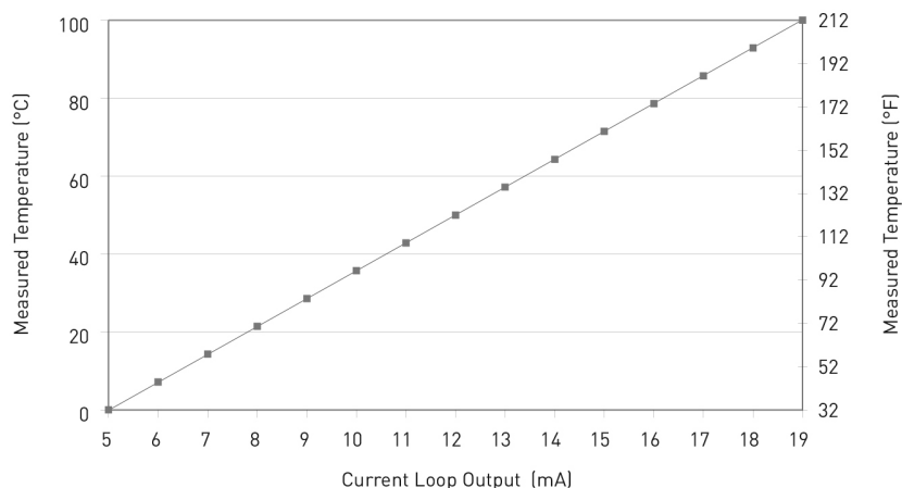
Figure 4.3: Temperature Control
