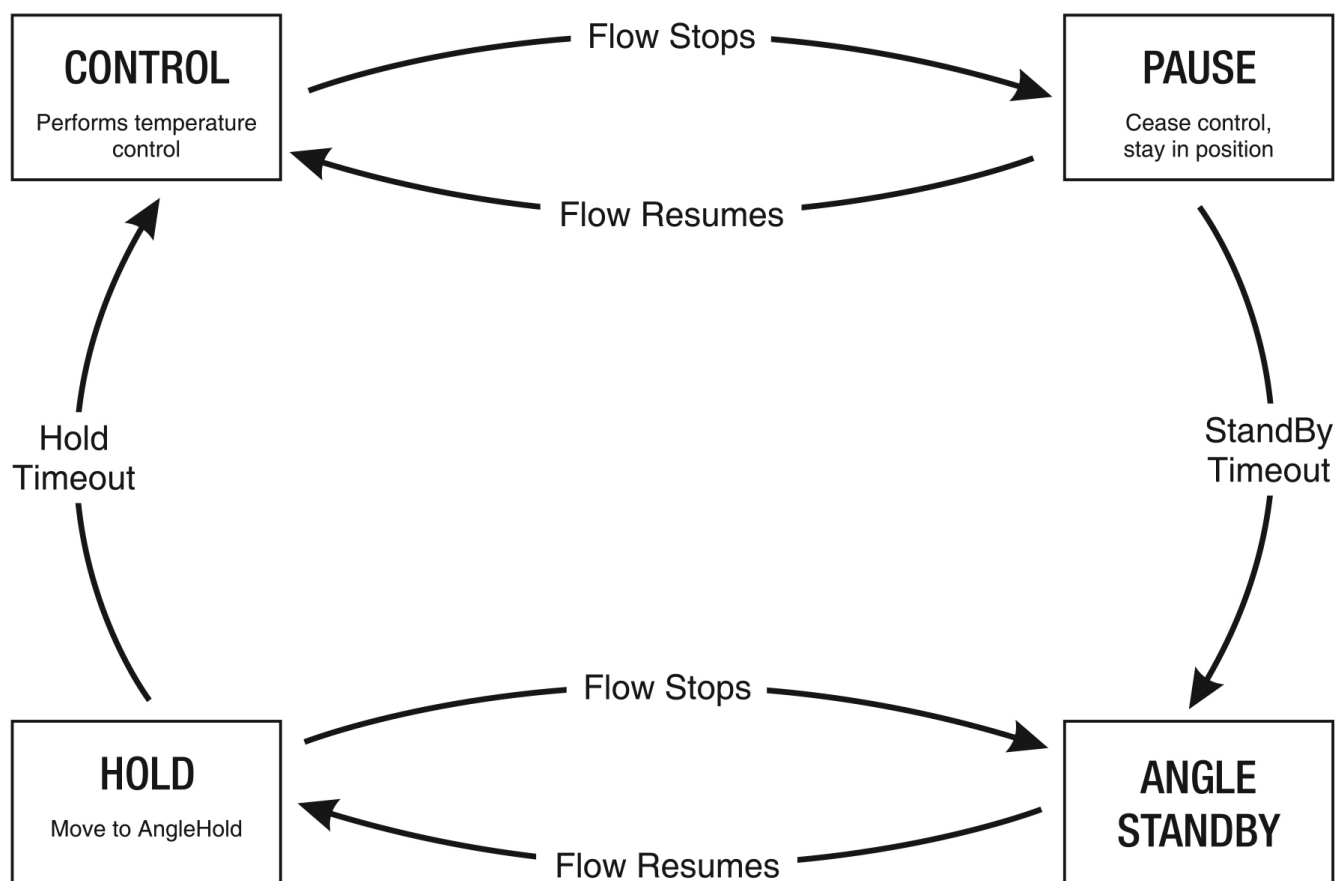
Figure 3.10: StandBy and Hold control cycle.
