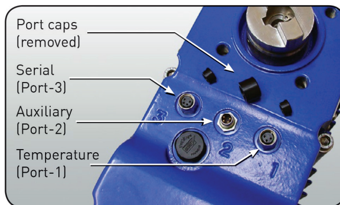
Figure 3.8: The underside of an Emech® G1 actuator showing the three port connectors.
